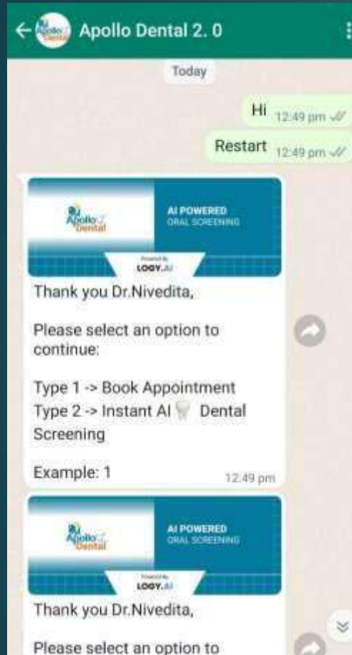
Normal chat
